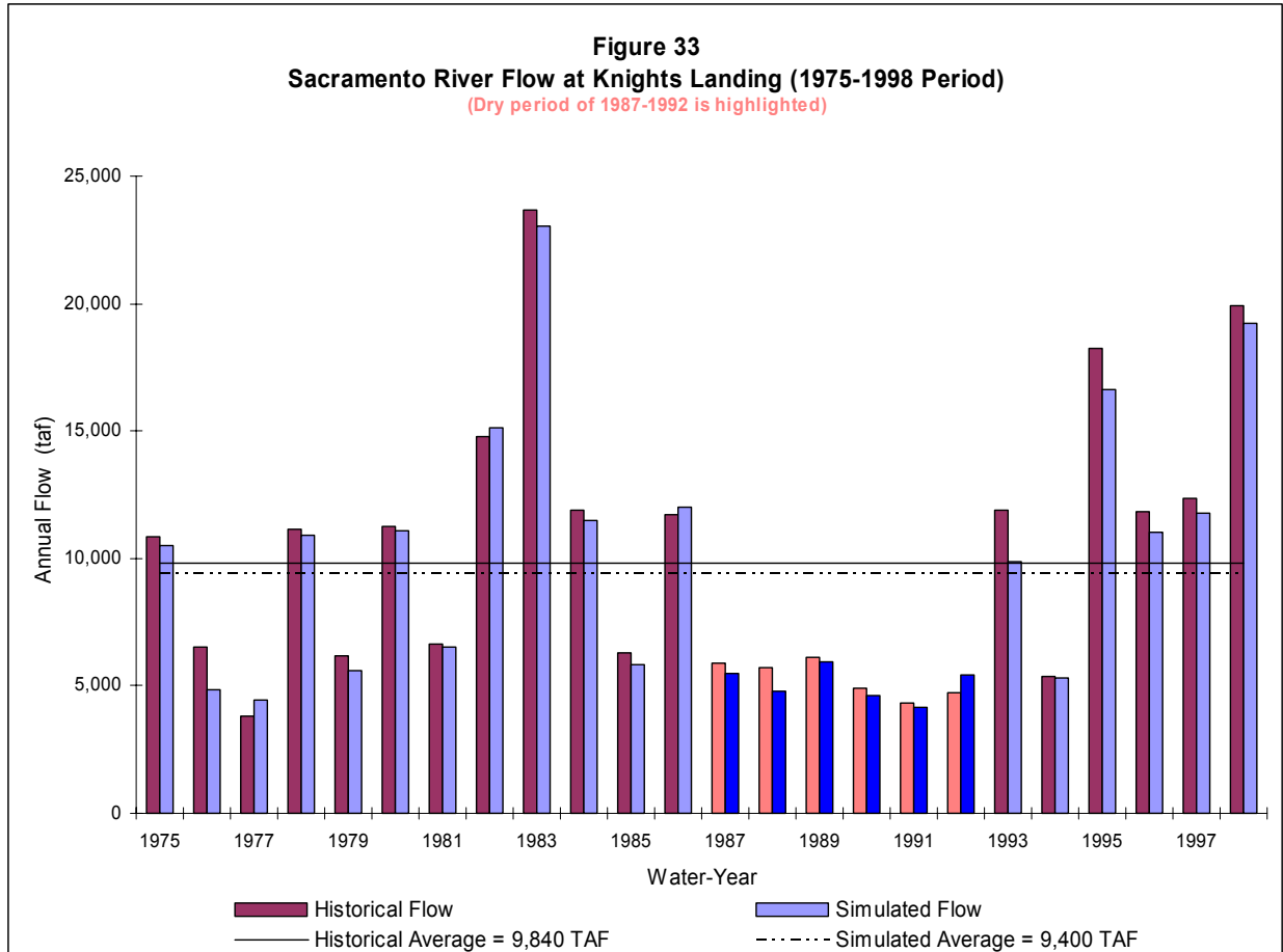
Figure 33 provides a comparison of the historical and simulated flows at the Knights Landing gaging station on the Sacramento River. The long-term average of the simulated values is lower than that of the historical values by about 4.5 percent. The historical average annual flow during the 6-year drought of 1987-1992 is about 5,290 taf per year. The average for the simulated values during the drought is 5,080 taf per year, a difference of about 4.0 percent.
