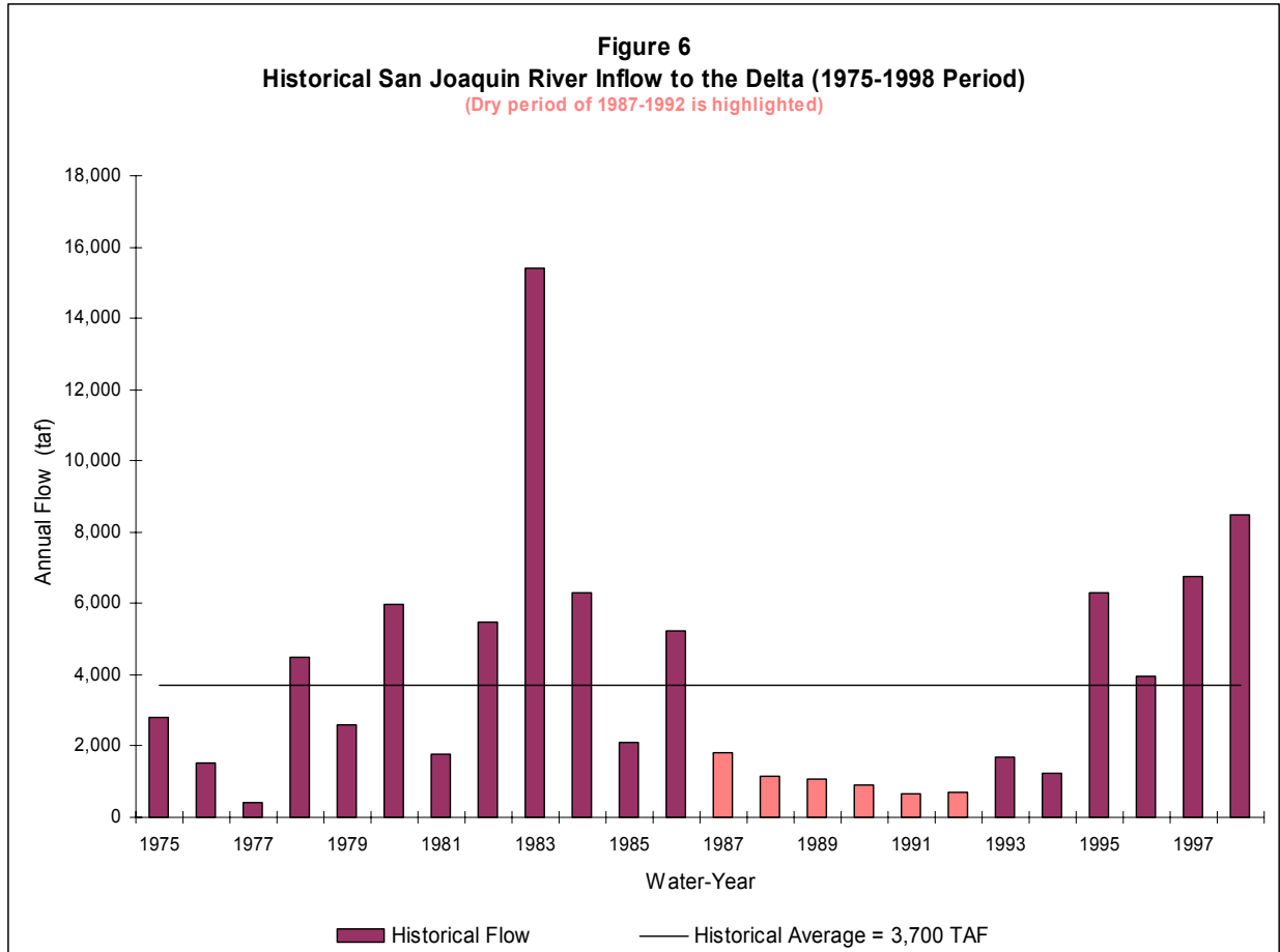
Figure 6 shows the historical inflow to the Delta from the San Joaquin River for the 1975-1998 period. These historical values were used in the Historical Operations Study for the CalSim II evaluation. The average annual inflow during the 6-year drought of 1987-1992 is about 1,050 taf per year.
