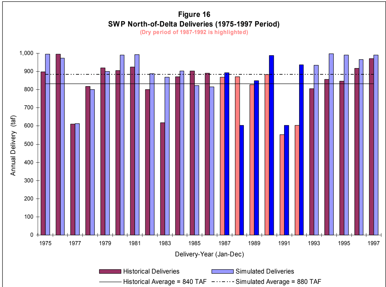
Figure 16 shows the bar chart of comparison between the historical and simulated deliveries made to SWP north-of-Delta contractors and senior water right holders in FRSA for the period of 1975-1997. The total includes deliveries made to all of the senior water rights holders downstream of Lake Oroville (i.e. Joint Water District Board, Western Canal Water District, Garden Highway Mutual Water Company, Plumas Mutual Water Company, Thermalito Irrigation District, Tudor Mutual Water Company, and Oswald Water District). The long-term average of the simulated deliveries exceeds that of the historical deliveries by approximately 4.8 percent. The historical average annual delivery during the 6-year drought of 1987-1992 is about 770 taf per year. The average for the simulated values during the drought is 810 taf per year, a difference of about 5.2 percent.
