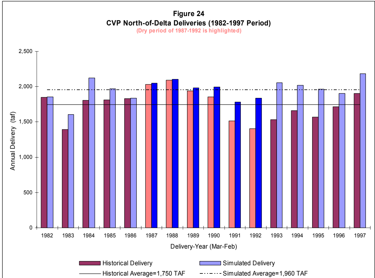
Figure 24 shows the bar chart of comparison between the historical and simulated deliveries made to the CVP north-of-Delta contractors in the Sacramento Valley for the period of 1982-1997. They include the Tehema-Colusa Canal service area, Corning Canal service area, Glenn-Colusa ID, Anderson-Cottonwood ID, City of Redding, Maxwell ID, Provident ID, Princeton-Codora-Glenn ID, Colusa IC, Meridian Farms WC, Pelger Mutual WC, RD 1004, RD 108, Roberts Ditch IC, Sartain MWD, Sutter MWC, Swinford Traft IC, Tisdale Irrigation and Drainage Company, and Sacramento, Delevan, and Colusa Refuge Areas. The long-term average of the simulated deliveries exceeds that of the historical deliveries by 12.0 percent. The historical average annual delivery during the 6-year drought of 1987-1992 is about 1,810 taf per year. The average for the simulated values during the drought is 1,960 taf per year, a difference of about 8.3 percent.
