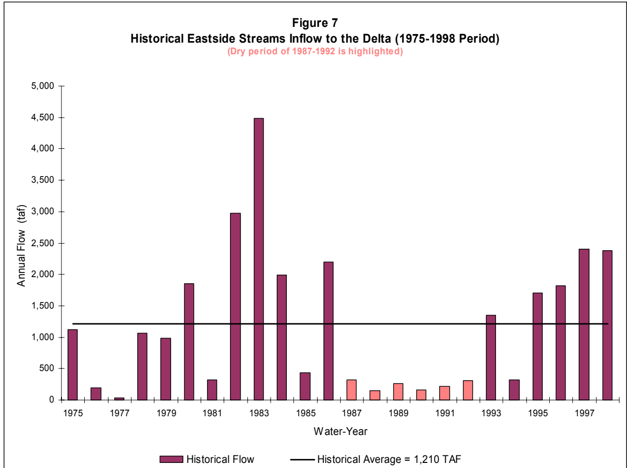
Figure 7 shows the historical inflow to the Delta from the Eastside Streams, including the Cosumnes, Mokelumne, and the Calaveras rivers for the 1975-1998 period. These historical values were used in the Historical Operations Study for the CalSim II evaluation. The average annual inflow during the 6-year drought of 1987-1992 is about 240 taf per year.
