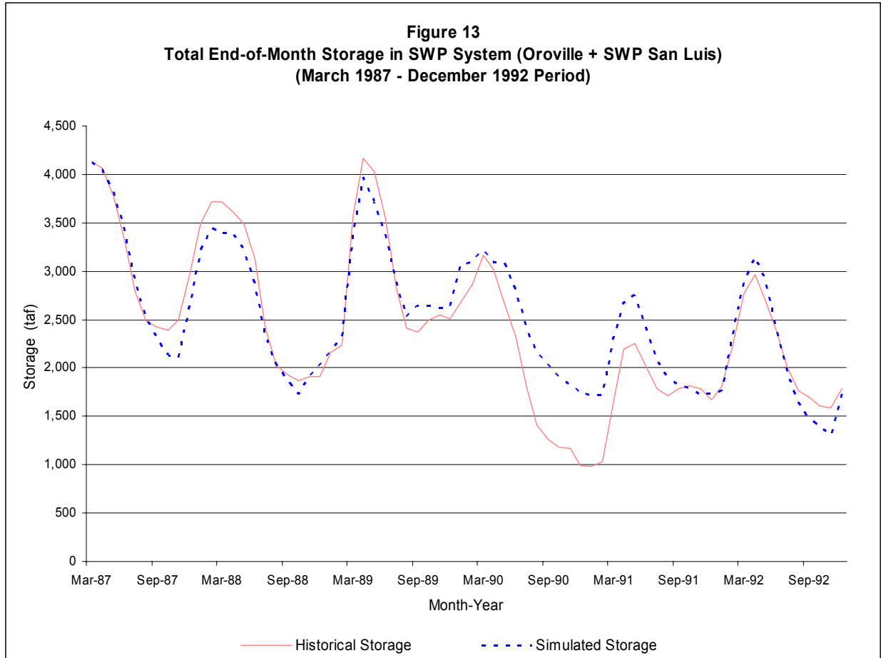
Figure 13 shows a line plot of the end-of-month SWP storage (Oroville plus SWP San Luis) for the 1987-1992 drought. The historical storage at the outset of the drought on March 31, 1987 was 4,139 taf. The corresponding storage marking the end of the drought on November 30, 1992 was 1,591 taf. The table below lists the storage values and the corresponding annual changes in storage for the beginning of each calendar year. The storage change for the first year of the drought was based on the end of March 1987 when the system storage was at its highest level before the drought began. Differences in the historical operation criteria and those used in the simulation study may result in different ending storages in SWP system. These storage differences were used to compute the adjustments for delivery bar charts presented in Figure 12.
