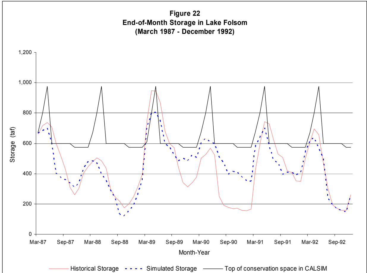
Figure 22 shows a plot of end-of-month storage in Lake Folsom for the 1987-1992 drought. The historical storage at the outset of the drought on March 31, 1987, was 662 taf. The corresponding marking the end of the drought on November 30, 1992, was 157 taf. The table below lists the storage values and the corresponding changes in storage for the beginning of each delivery year. The storage change for the first year of the drought was based on the end-of-March 1987 when the system storage was at its highest level, just before the drought began.
