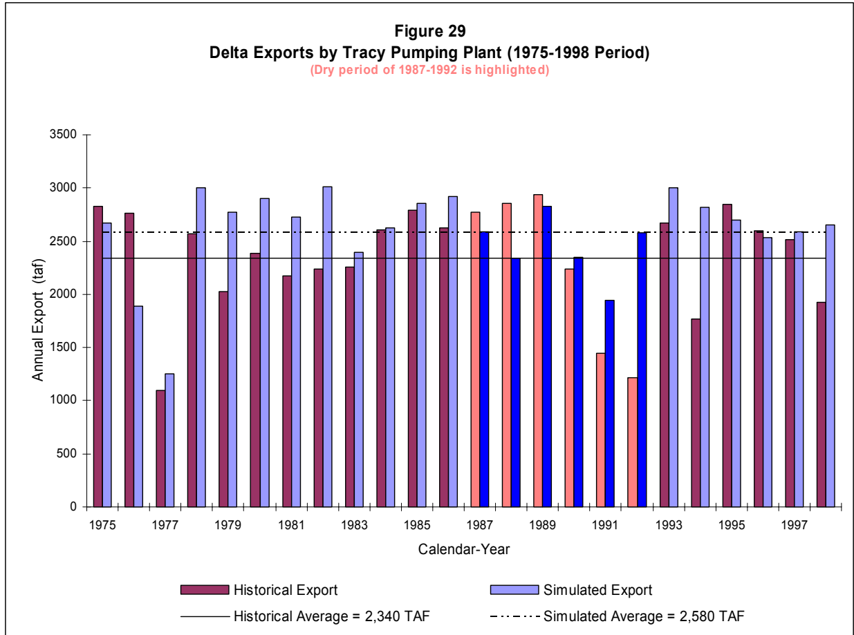
Figure 29 shows the total exports made from the Delta by the Tracy Pumping Plant. Historical values were obtained from DAYFLOW. The simulated long-term average annual exports exceeded the historical average by approximately 10.3 percent.
