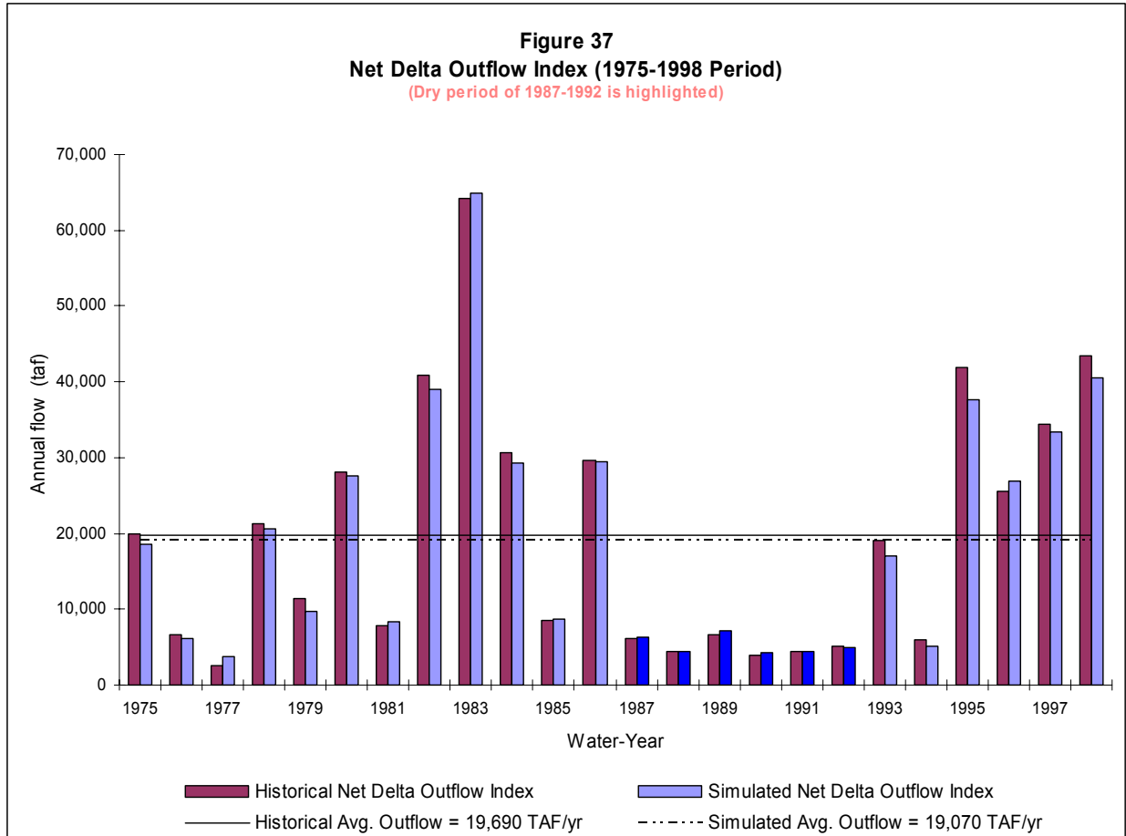
Figure 37 presents a comparison between the historical and simulated values of the Net Delta Outflow Index. Historical values of the NDOI were obtained from DAYFLOW, which estimates this variable by performing a water balance at the boundary of the Sacramento-San Joaquin Delta, taking Chipps Island as the western limit. The long-term average of the simulated values is lower than that of the historical values by about 3.1 percent. The historical average annual outflow during the 6-year drought of 1987-1992 is about 5,090 taf per year. The average for the simulated values during the drought is 5,270 taf per year, a difference of about 3.5 percent.
