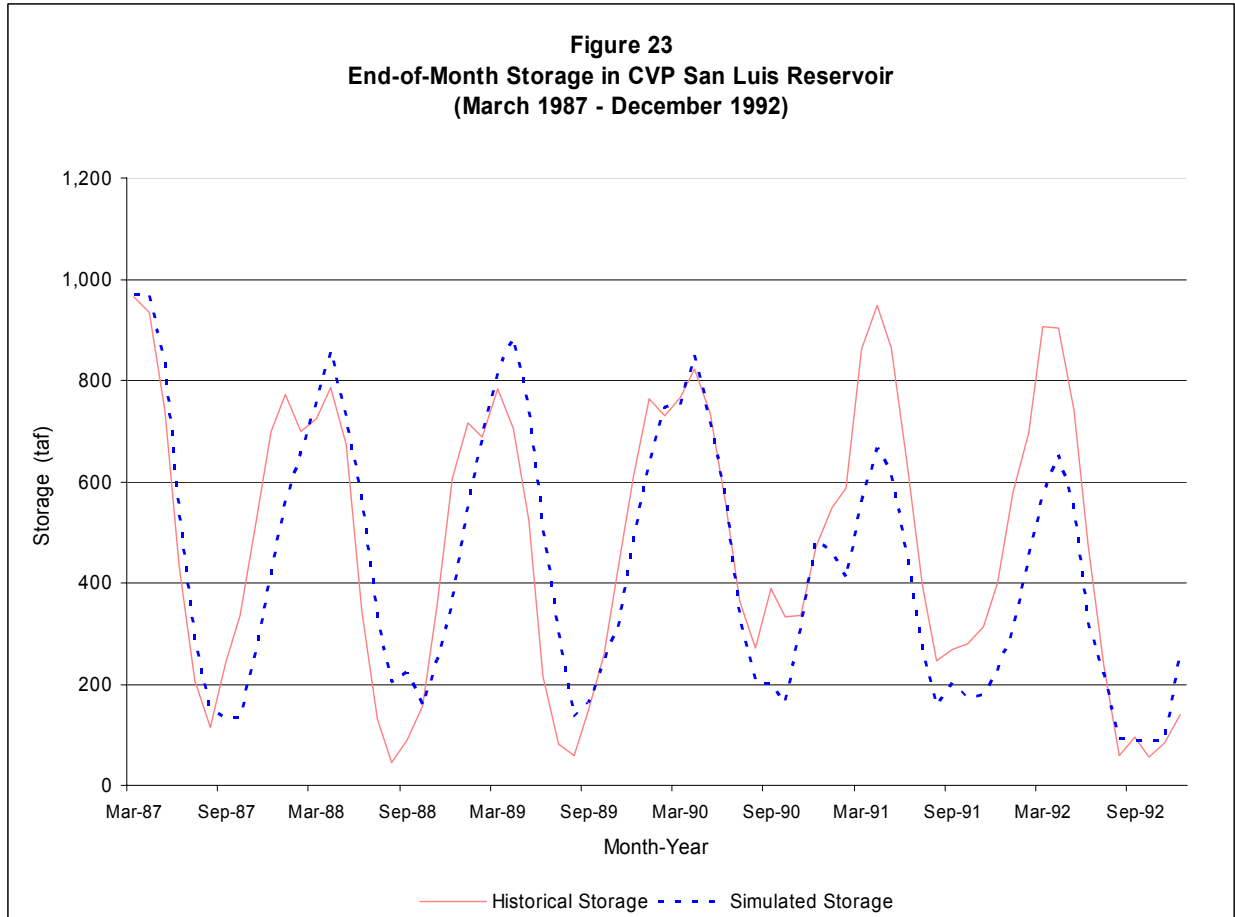
Figure 23 shows a plot of end-of-month storage in CVP San Luis Reservoir for the 1987-1992 drought. The historical storage at the outset of the drought on March 31, 1987, was 964 taf. The corresponding storage marking the end of the drought on October 31, 1992, was 57 taf. The table below lists the storage values and the corresponding changes in storage for the beginning of each delivery year. The storage change for the first year of the drought was based on the end-of-March 1987 when the system storage was at its highest level, just before the drought began.
