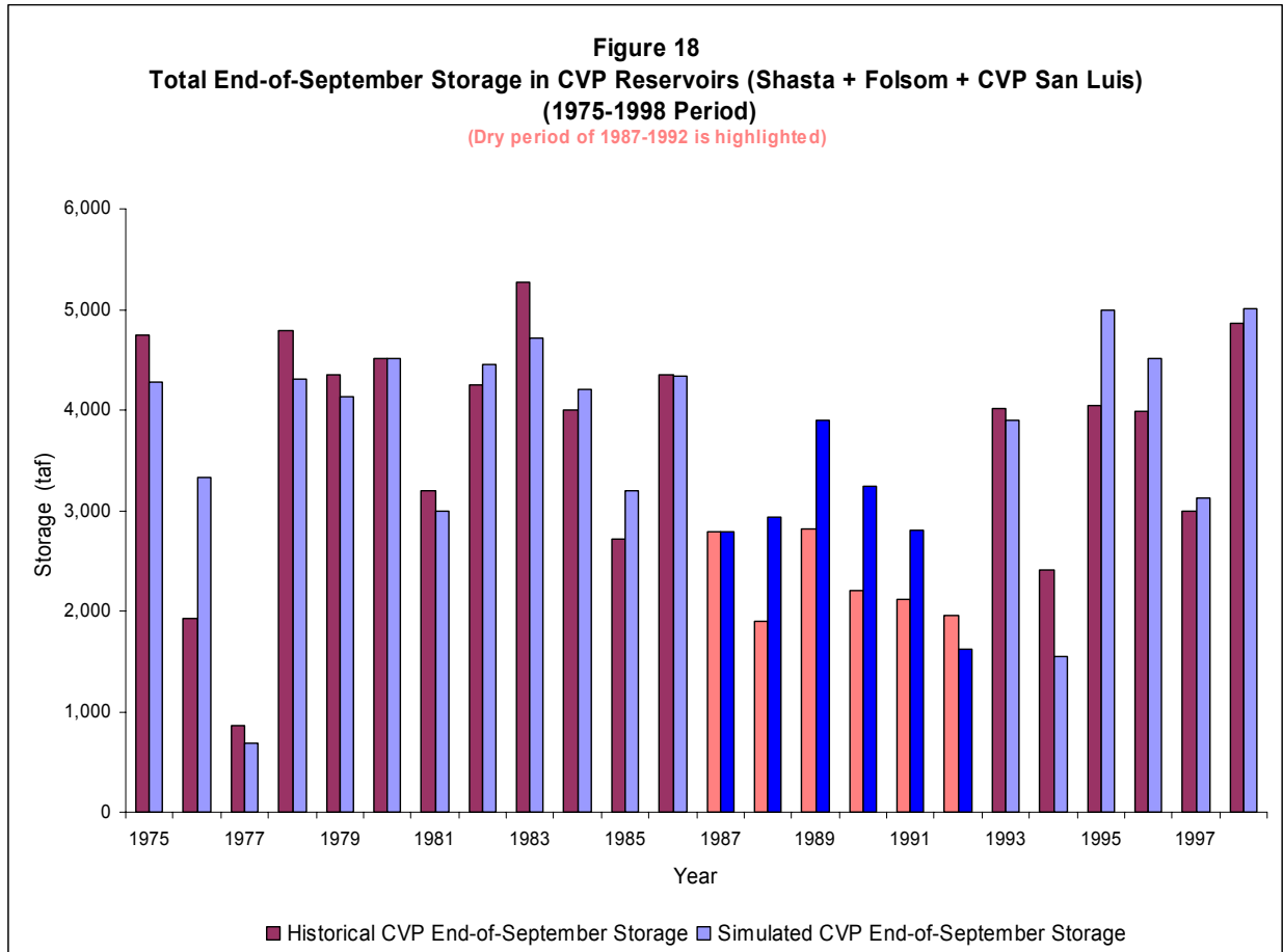
Figure 18 shows the total storage in the CVP system (Shasta, Folsom, CVP San Luis) reservoirs at the end of each water year. System carryover storage at the end of the water year is one of the factors that determine the allocation of water for making deliveries to CVP contractors.
