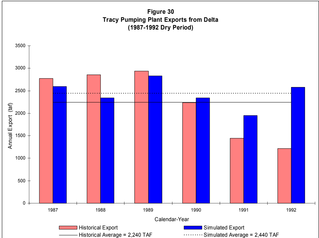
Figure 30 shows the total exports made from the Delta by the Tracy Pumping Plant during the dry period of 1987-1992. Historical values were obtained from DAYFLOW. The historical average annual export during the 6-year drought is about 2,240 taf per year. The average for the simulated values during the same period is 2,440 taf per year, a difference of about 8.9 percent.
