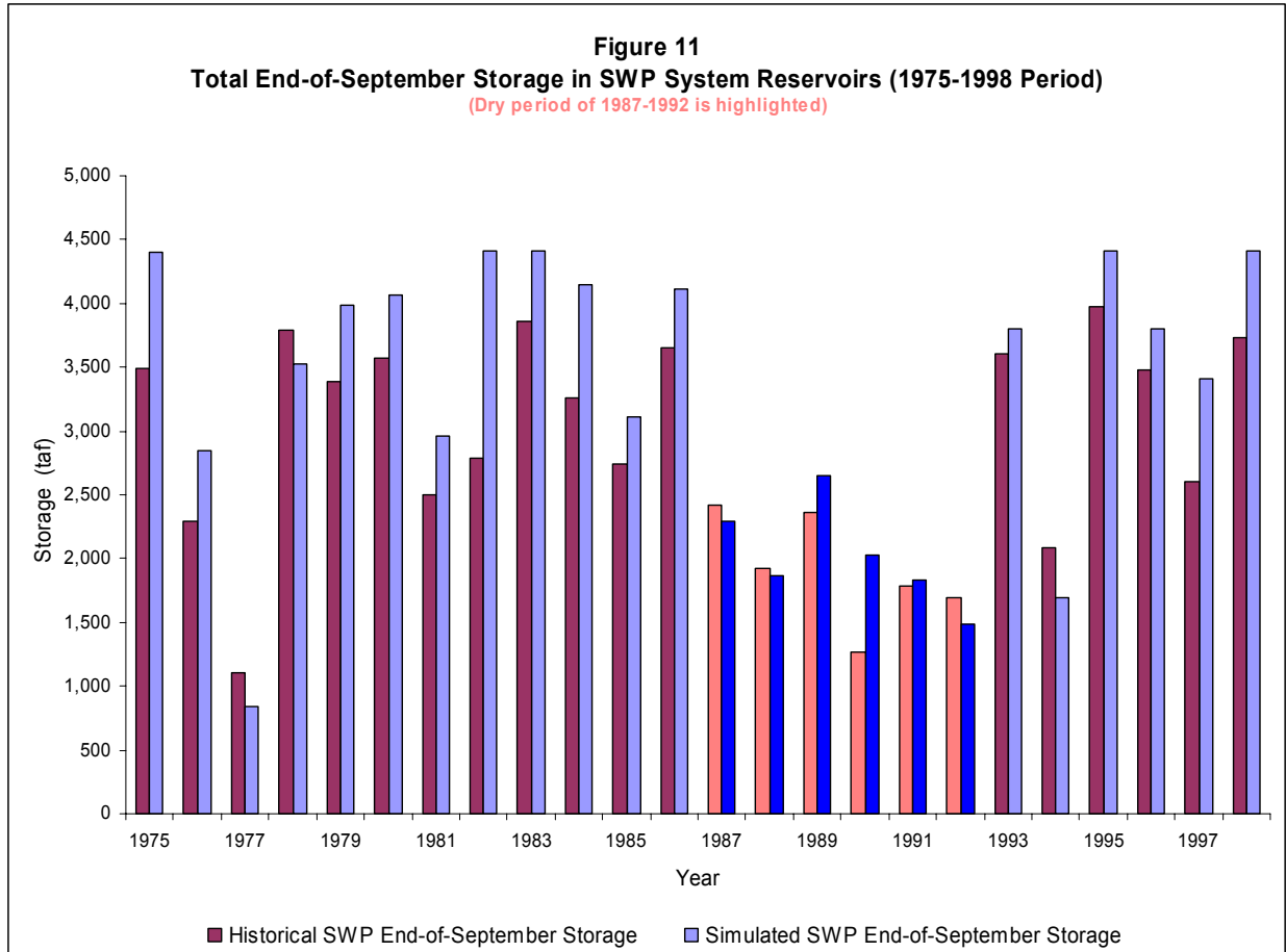
Figure 11 shows the total storage in the SWP system reservoirs at the end of each water year. The carryover storage in the system (Lake Oroville + SWP San Luis Reservoir) is one of the factors that determine the SWP allocations.
