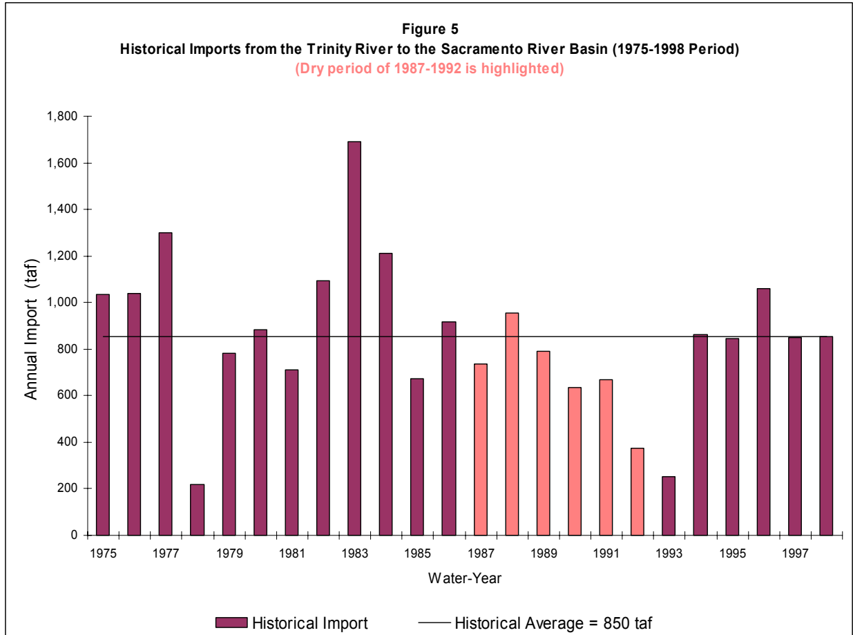
Figure 5 shows the historical imports through the Clear Creek Tunnel for the 1975-1998 period used in the Historical Operations Study for the CalSim II evaluation. The average annual import during the 6-year drought of 1987-1992 is about 670 taf per year.
