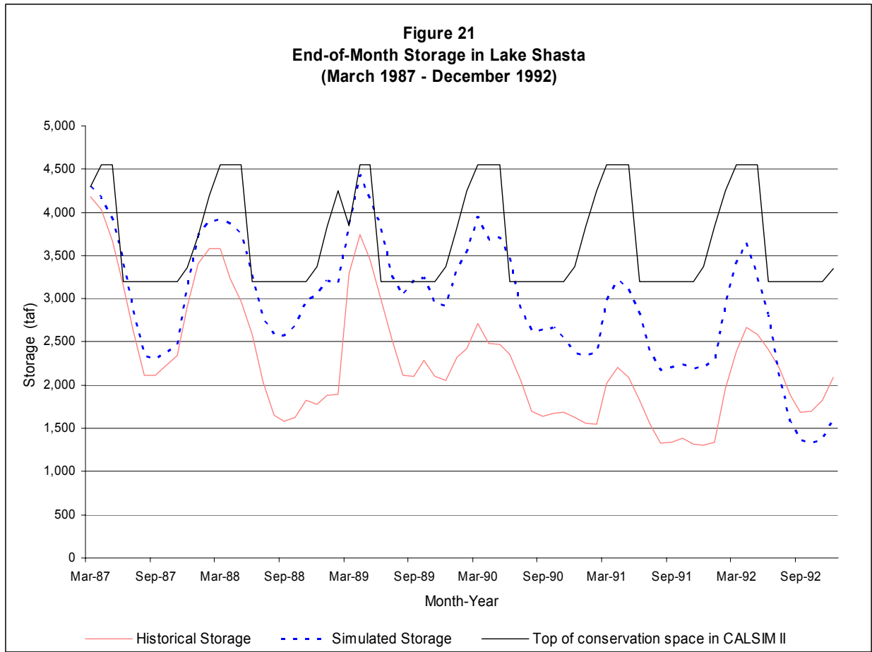
Figure 21 shows a plot of end-of-month storage in Lake Shasta for the 1987-1992 drought. The historical storage at the outset of the drought on March 31, 1987, was 4,182 taf. The corresponding storage marking the end of the drought on September 30, 1992, was 1,683 taf. The table below lists the storage values and the corresponding changes in storage for the beginning of each delivery year. The storage change for the first year of the drought was based on the end-of-March 1987 when the system storage was at its highest level, just before the drought began.
