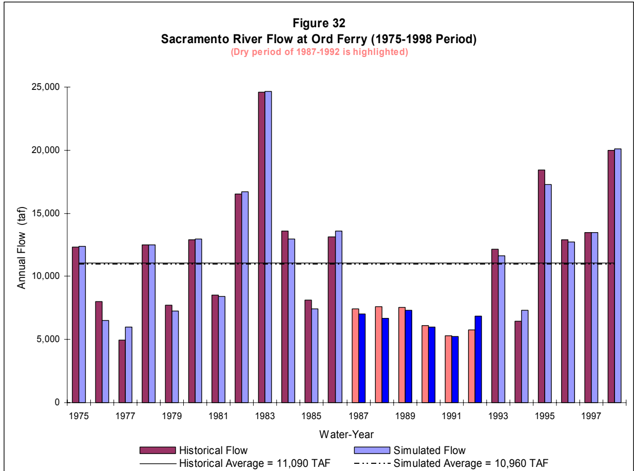
Figure 32 provides a comparison of the historical and simulated flows at the gaging station near Ord Ferry on the Sacramento River. The long-term average of the simulated values is lower than that of the historical values by about 1.2 percent. The historical average annual flow during the 6-year drought of 1987-1992 is about 6,620 taf per year. The average for the simulated values during the drought is 6,510 taf per year, a difference of about 1.7 percent.
