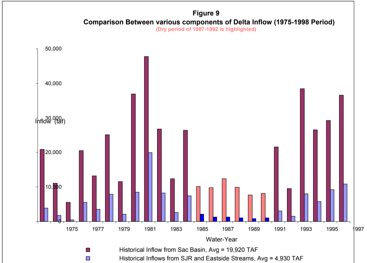
Figure 9 shows a comparison between the historical inflow to the Delta from the combined San Joaquin River and the Eastside Streams and the historical Delta inflow from the Sacramento Basin. The long-term average of the inflows from the San Joaquin River and the Eastside Streams are about 24.8 percent of the historical Delta inflow from the Sacramento Basin. The historical average annual inflow from the Sacramento Valley during the 6-year drought of 1987-1992 is about 9,670 taf per year. The average for the historical inflow from the San Joaquin Basin and the Eastside Streams during the drought is 1,340 taf per year, about 13.9 percent of the inflow from the Sacramento Basin.
