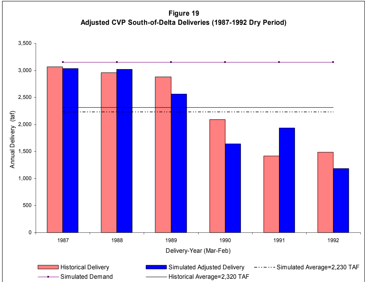
Figure 19 shows a comparison of historical and simulated CVP deliveries to south-of-Delta contractors during the 1987-1992 drought. Simulated annual deliveries during the drought have been adjusted to account for the difference in storage utilization in any given year. After the corrections for storage utilization during the critical period the 6-year average of the simulated deliveries is lower than that of the historical deliveries by approximately 3.9 percent. The adjusted simulated deliveries shown in this bar chart are computed as the gross delivery for each delivery year of simulation minus the difference between the historical and simulated values of storage used from March 1 to February 28(29) of the following year. For the first year of the drought, 1987, the storage difference between March 31 (the highest system storage just before the onset of the drought) and February 29, 1988, was used. Storage differences are based on the total CVP system storage (Shasta, Folsom, and CVP San Luis).
