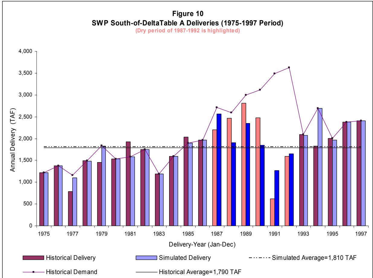
Figure 10 shows a comparison of historical and simulated SWP deliveries to south-of-Delta contractors for calendar years 1975 to 1997. Simulated deliveries in 1981 and 1985 are lower than historical deliveries due to the lower initial contractors requests used as demands for those years according to the rules discussed in Section 4.4.3. The higher historical deliveries, however, indicate that there might have been a revision in contractors’ requests for higher deliveries subsequent to their submission of initial requests. Long-term average of the simulated deliveries exceeds that of the historical deliveries by approximately 1.1 percent. Both historical and simulated deliveries include only Table A deliveries without any Article 21 or any non-project deliveries.
