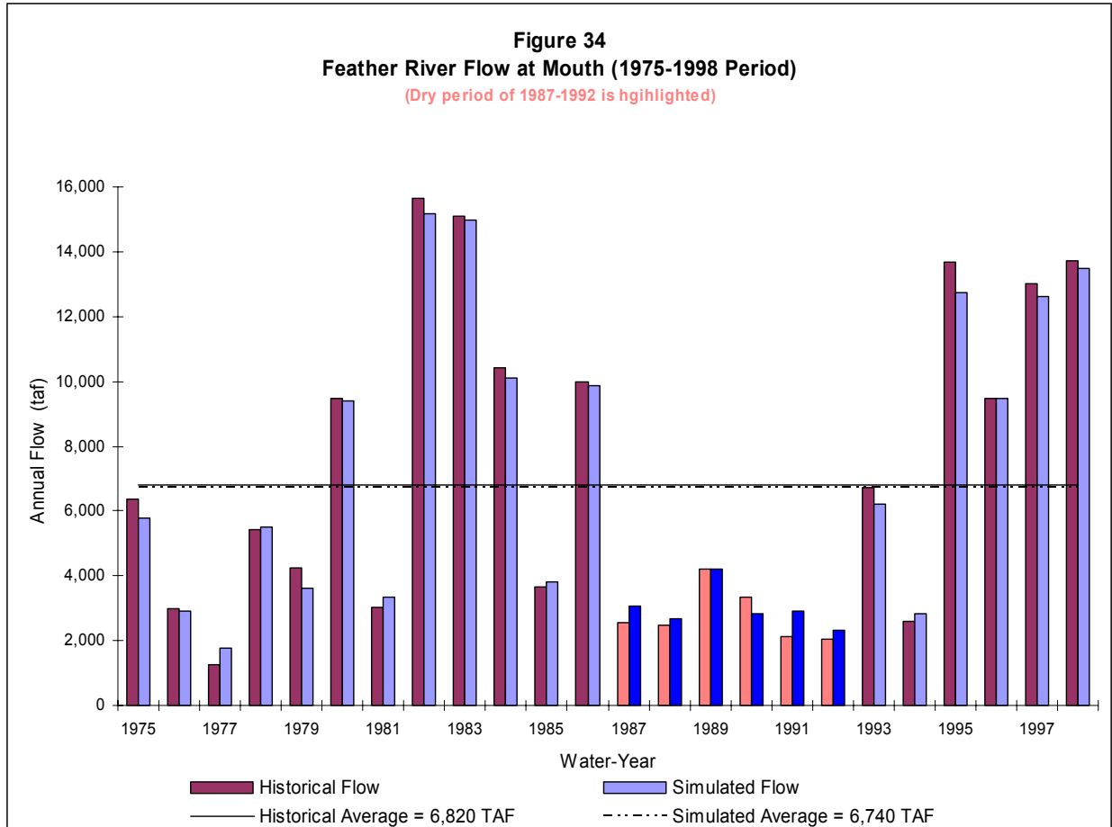
Figure 34 provides a comparison of the historical and simulated flows in the Feather River at confluence with the Sacramento River. The long-term average of the simulated values is lower than that of the historical values by about 1.2 percent. The historical average annual flow during the 6-year drought of 1987-1992 is about 2,800 taf per year. The average for the simulated values during the drought is 3,000 taf per year, a difference of about 7.1 percent.
